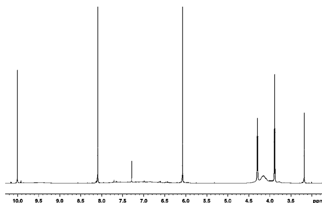
Figure 1. 1 H NMR spectrum of compound 2 (CDCl 3 , 298 K, 600 MHz).
