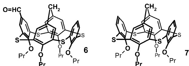
Figure 5. Intermediates isolated from the Duff reaction.
