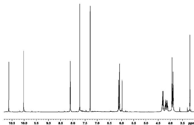
Figure 3. 1 H NMR spectrum of compound 3 (CDCl 3 , 298 K, 600 MHz).
