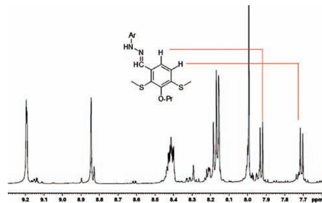
Figure 4. Partial 1 H NMR spectrum of compound 3a (CDCl 3 , 298 K, 600 MHz).
